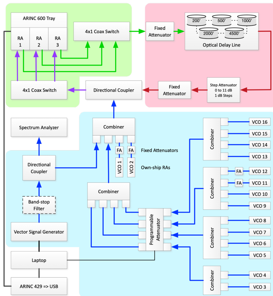
Figure 2-1: AVSI Test Schematic
