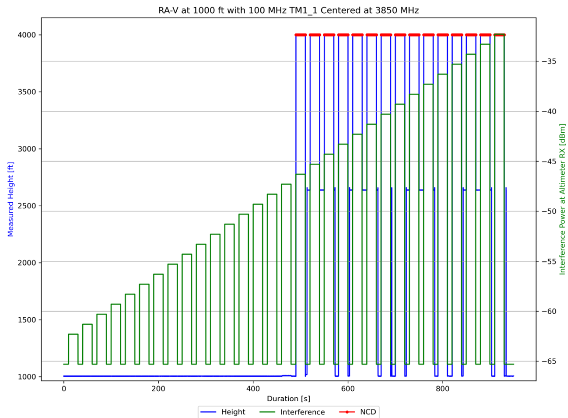
Figure 3-174: UC2 RA-V 1000' AGL Time History with TM1.1 at 3850 MHz
