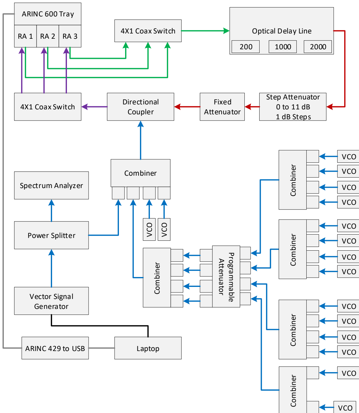
Figure 3: Block Diagram of the Test Setup.
